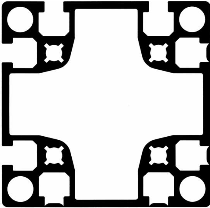
Part No. 20.1044/0
