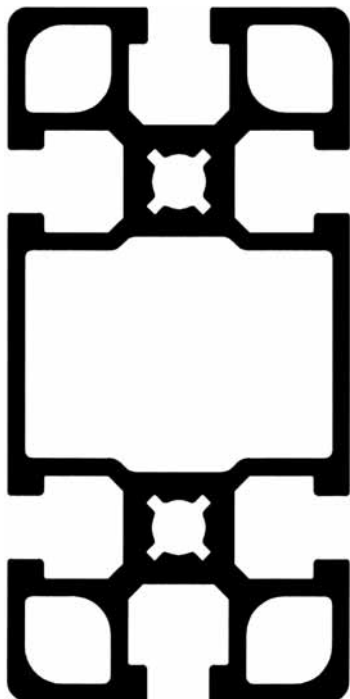
Part No. 20.1032/0
