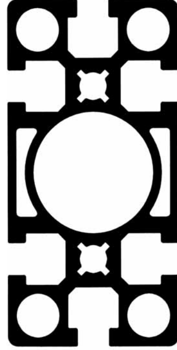
Part No. 20.1017/0
